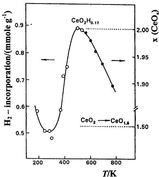
Figure 24. Mass changes of a \text{CeO}_2 sample subjected to \text{H}_2 treatments, (O) \text{H}_2 incorporation at constant \text{H}_2 pressure (70 torr); (●), average degree of reduction given by the O/Ce ratio ( \text{CeO}_x ).
