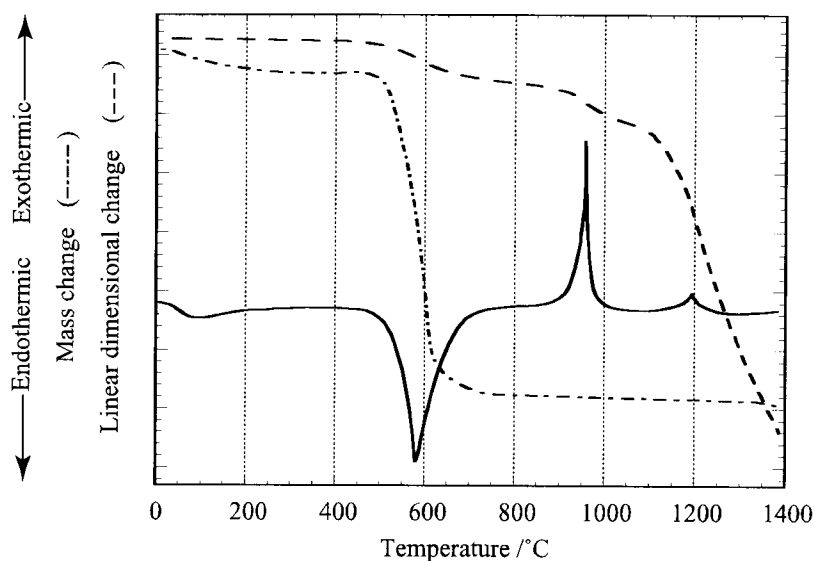
Figure 4. DTA, TG, and dilatometry curves for a kaolinite specimen [6]. Thermodilatometry is discussed in Chapter 6 of Volume 1 of this Handbook.
