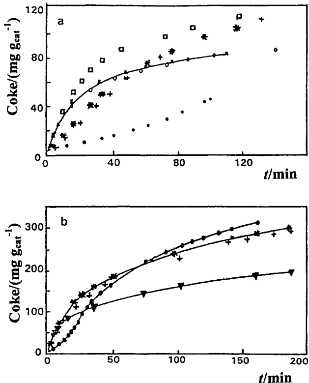
Figure 29. Coke deposition from propane (a) and propene (b) onto \text{Cr}_2\text{O}_3 catalysts pre-reduced by CO: (●), 0.0 %; (+), 1.5 %; (★), 3.0; (□), 6.0; (◇), 12.0; (▼) 15.0 % of \text{Cr}_2\text{O}_3 .
