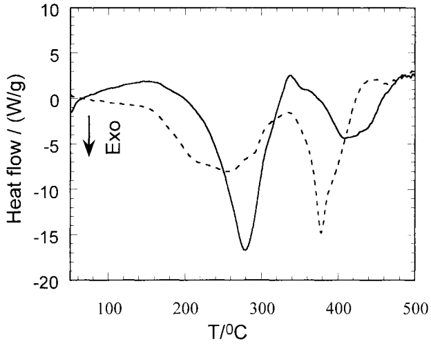
Figure 1. DSC oxidative degradation curves from two locations on the 16 th century painting by F. di Giorgio Martini, egg tempera based medium (—) and oil-based medium (---) [33].
