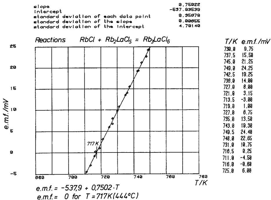
Figure 7b. Emf vs T curve for Rb_3LaCl_6 [55a].
