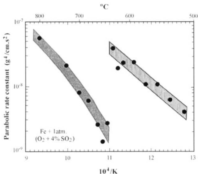
Figure 38. The parabolic rate constant for the corrosion of iron in O 2 + 4% SO 2 as a function of reciprocal absolute temperature; note the discontinuity at about 640 °C. From A. Holt and P. Kofstad, reference 100.
