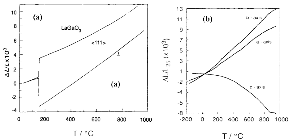
Figure 34 - Thermal expansion of single crystals through a phase transformation. (a) \text{LaGaO}_3 parallel and orthogonal to the 111 - axis [50] (b) along the c-axis for \text{KTiOAsO}_4 [51].
