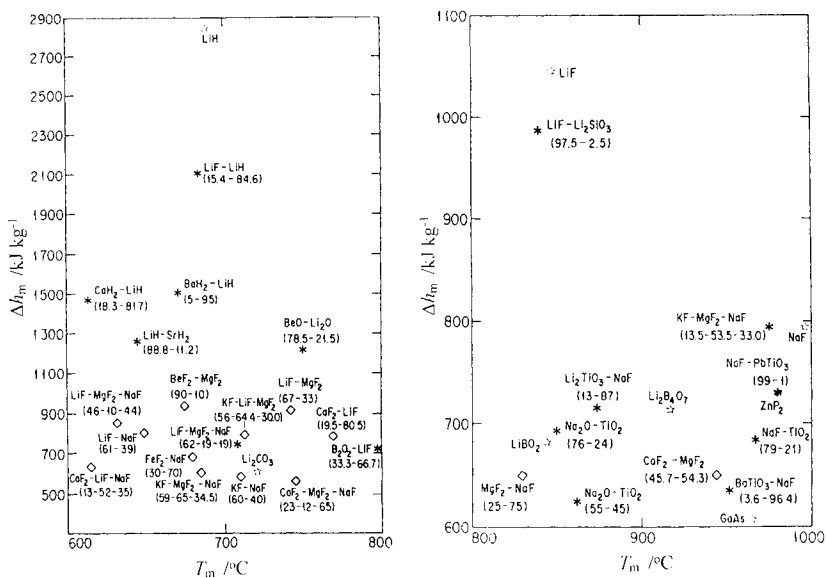
Figure 3. Temperatures of fusion and latent heats of promising latent thermal storage materials above 600 °C [6].
