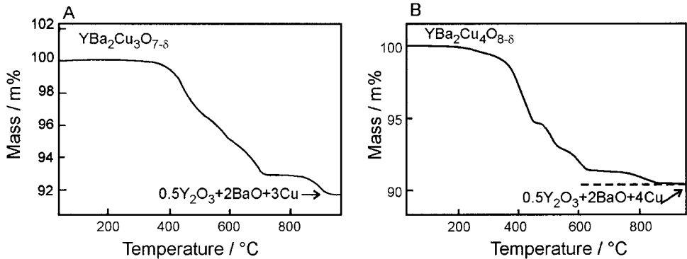
Figure 18. Hydrogen reduction curves of (A) YBa 2 Cu 3 O 7.8 [after 196] and (B) YBa 2 Cu 4 O 8.8 [199] heating rate 5 °C min -1 .
