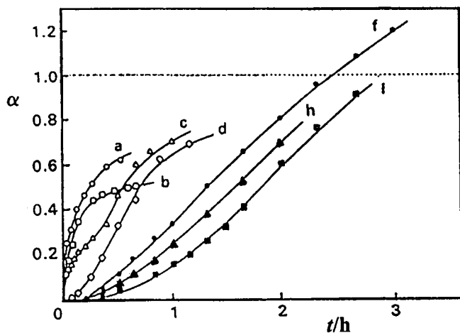
Figure 19. Kinetics of reduction of Mo-Pr-O catalysts: (Mo/(Mo+Pr) = 0.0, (a); 0.09, (b); 0.27, (c); 0.43, (d); 0.80, (e); 0.88, (f); 0.91, (g); 0.95, (h); 1.0, (i)) in a flow of 50 \text{ cm}^3 \text{ min}^{-1} \text{ H}_2 at 773 K.
