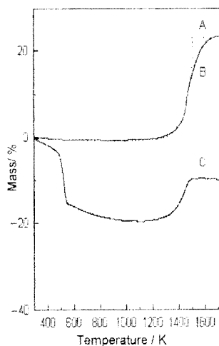
Figure 40. TG curves for samples of AlN heated in air [66].
