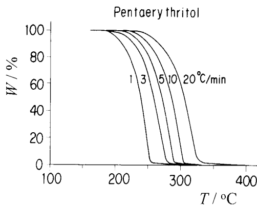
Figure 21. TG curves of pentaerythritol heated in nitrogen in shallow open sample pans at the indicated heating rates [8]. W : Residual mass %.
