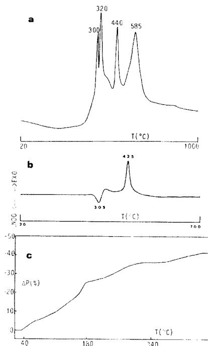
Figure 70. Thermoanalytical curves associated with the decomposition of a titania xerogel doped with Cr 3+ and Al 3+ [116].
