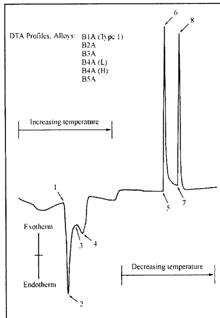
Figure 17. DTA curve for the borated stainless steel alloy 304B2A. The curve is representative of the behavior of alloys B1A through B5A. From C.V. Robino and M.J. Cieslak, reference 56.
