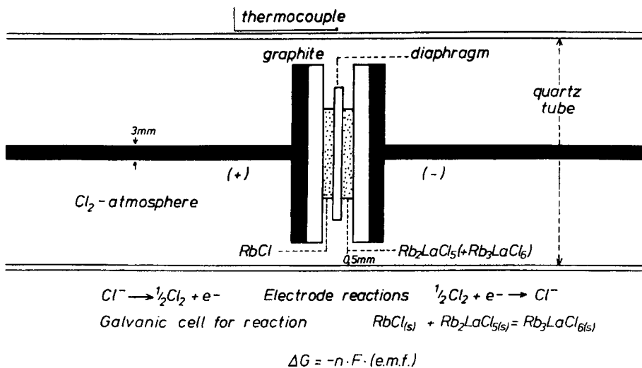
Figure 7a. Galvanic cell for the reaction: RbCl + Rb_2LaCl_5 = Rb_3LaCl_6 [55a].
