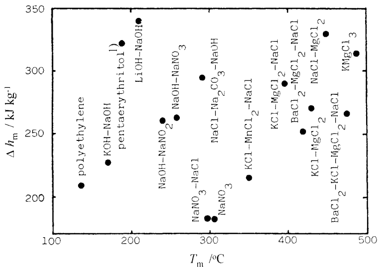
Figure 2. Temperatures of phase changes and latent heats of promising latent thermal storage materials between 100 °C and 500 °C [5].
