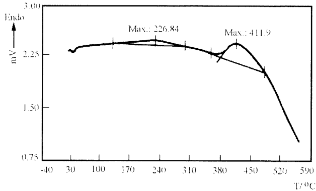
Figure 50. DSC curve for a normalized Al/SiC sample; heating rate 20 \text{ deg min}^{-1} . From J.P. Hébert and E. Karmazsin, reference 203.
