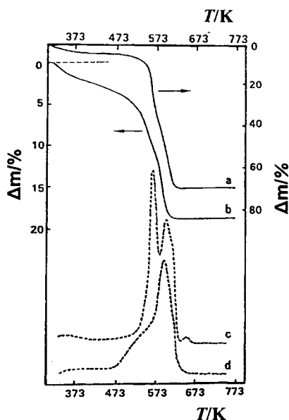
Figure 1. (a) TG of \text{H}_2[\text{VO}(\text{C}_2\text{O}_4)_2] \cdot \text{H}_2\text{O} at 277 \text{ K min}^{-1} in dry \text{N}_2 ; (b) TG of the precursor under the same experimental conditions; (c) time-temperature derivative of TG curve (a); (d) time-temperature derivative of TG curve (b).
