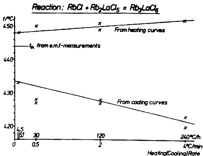
Figure 6. Hysteresis for the formation/decomposition temperature of Rb_3LaCl_6 [55c].
