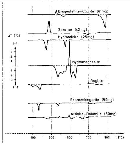
Figure 49. DTA curves of hydrated carbonates with other anions, e.g. brugnatelite, zaratite, hydrotalcite, hydromagnesite, voglite, schrockingerite, and artinite.
