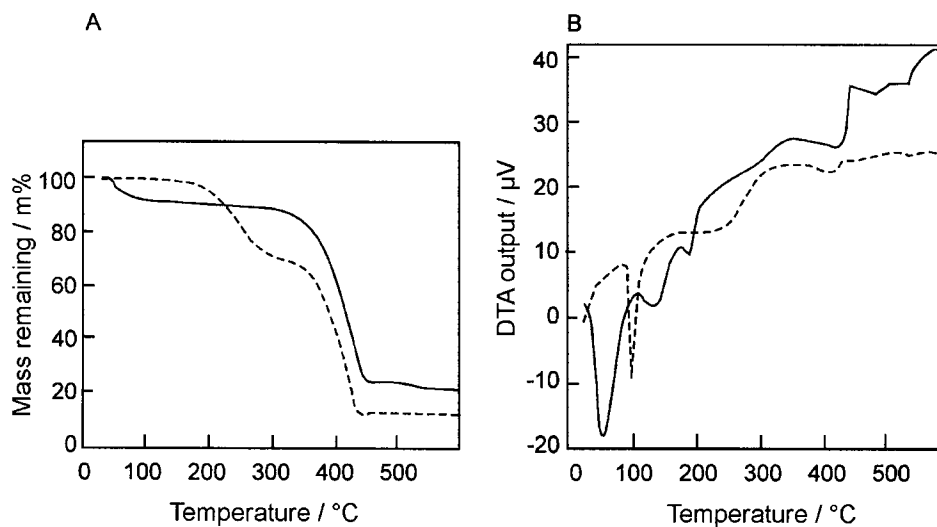
Figure 21. (A) TG and (B) DTA curves recorded in a flowing Ar atmosphere, heating rate 10\text{ }^{\circ}\text{C min}^{-1} , for ten-week-old commercial samples of "Ba(thd) 2 " (—) and [Ba(thd) 2 (tetraglyme)] (---) [after 241].
