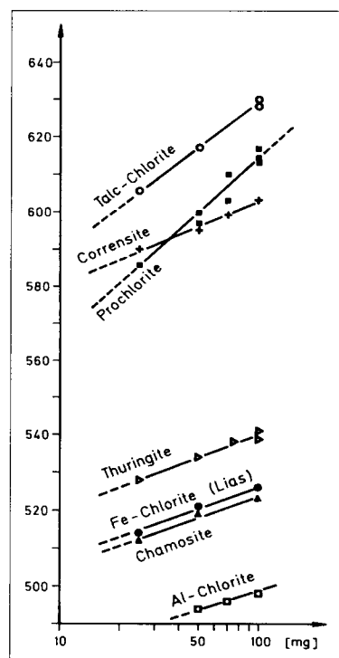
Figure 32. PA-curves of chlorites and corrensite.
