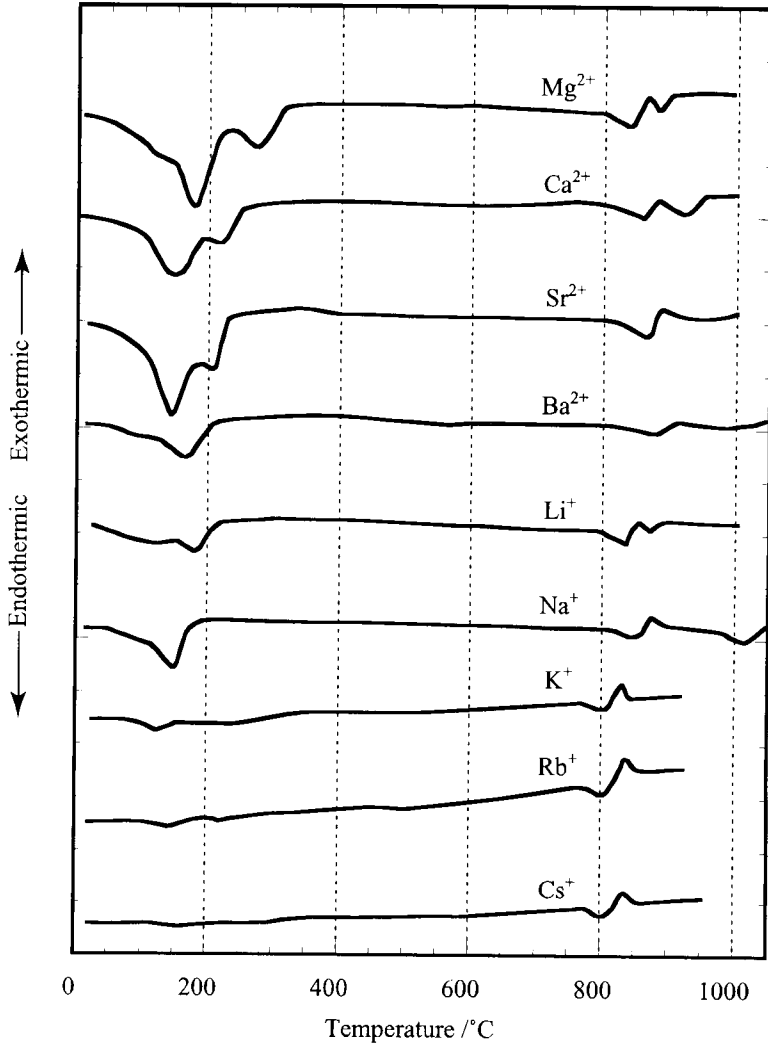
Figure 19. DTA traces of vermiculites saturated with the indicated exchangeable cations. \text{Mg}^{2+} , \text{Ca}^{2+} , \text{Sr}^{2+} , \text{Ba}^{2+} , \text{Li}^+ , \text{Na}^+ vermiculite samples are from a West Chester, PA deposit, while \text{K}^+ , \text{Rb}^+ , and \text{Cs}^+ samples are from a Macon County, North Carolina deposit [17].
