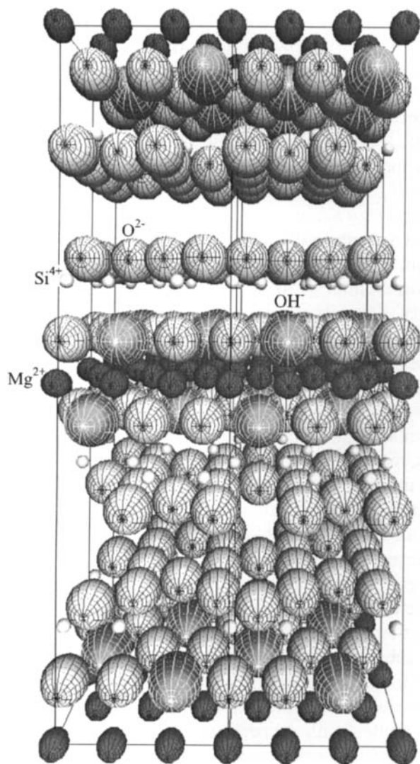
Figure 7. The structure of talc. Talc has a similar structure to pyrophyllite, in which Mg^{2+} replaces Al^{3+} , and additional Mg^{2+} ions are placed in the Mg^{2+} sheets to maintain space charge neutrality.
