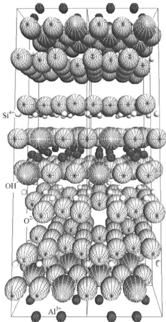
Figure 6. The structure of pyrophyllite. Montmorillonite clay minerals are based on the structure of pyrophyllite with cation substitutions for Al 3+ and Si 4+ .
