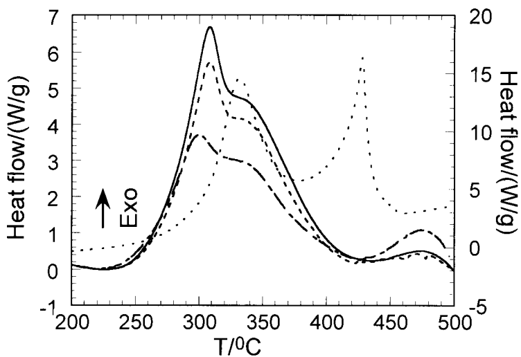
Figure 7. DSC oxidative degradation curves of control (—), light aged 64 hrs (--) and historical 16 th century silk fibres, “Jupiter and Ganimeses” (Brussels 1545) collection Royal Palace in Madrid (— --), and synthetic fibre (...).
