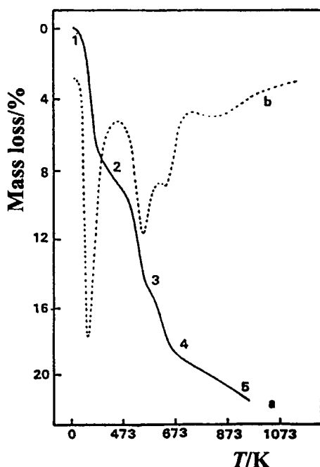
Figure 6. (a) TG curve of \text{Sc}(\text{OH})_3 xerogel decomposition in dry nitrogen at a heating rate of 5\text{ K min}^{-1} . (b) Time-temperature derivative of TG curve (a).
