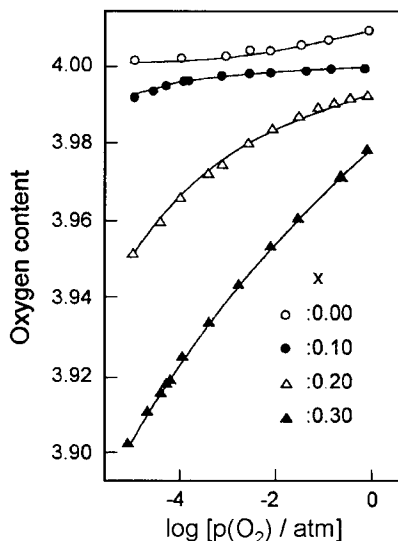
Figure 9. Oxygen content of \text{La}_{2-x}\text{Sr}_x\text{CuO}_{4.6} as a function of p(\text{O}_2) and Sr content ( x ) at 900^\circ\text{C} [after 127].
