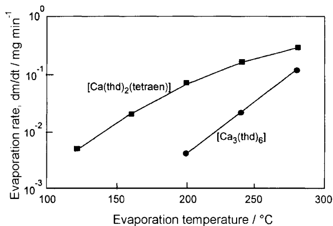
Figure 23. Evaporation rates of [Ca_3(thd)_6] and [Ca(thd)_2(tetraen)] as a function of temperature [after 264]. thd = 2,2,6,6-tetramethylheptane-3,5-dione, tetraen = tetraethylenepentamine.
