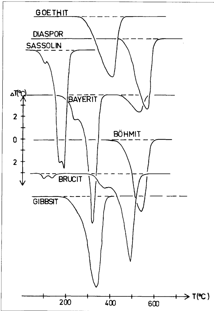
Figure 11. DTA curves of the hydroxides: goethite, diaspor, sassolite, bayerite, boehmite, brucite, and gibbsite.
