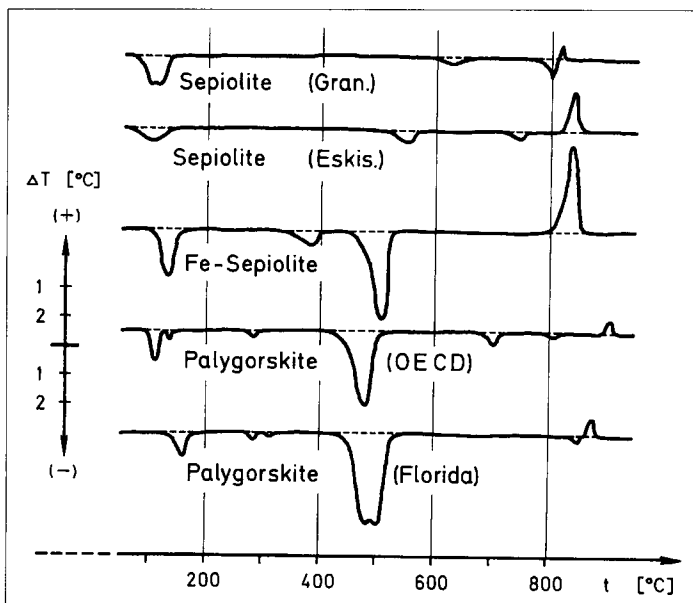
Figure 34. DTA curves of palygorskite and sepiolite.
