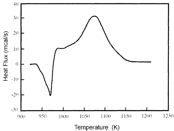
Figure 47. Non-isothermal DSC curve for the formation of TiAl_3 from titanium and aluminum powders; heating rate 30 \text{ K min}^{-1} , particle size < 45 \mu\text{m} . From X. Wang et al., reference 194.
